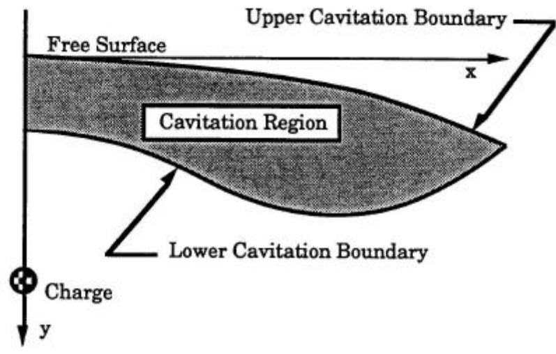
Figure 4. Bulk Cavitation Zone [Ref. 6]
