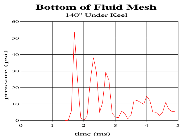
Figure 59. 3-D Model w/Offset Charge Fluid Mesh Pressure Profiles
