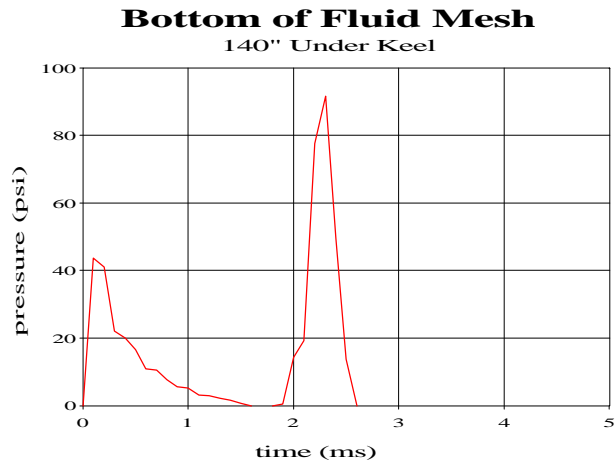
Figure 30. 2-D Model w/Charge Under Keel Fluid Mesh Pressure Profiles
