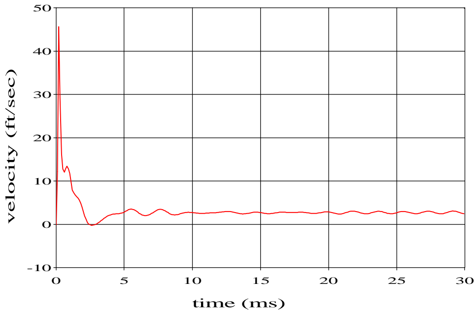
Figure 34. 2-D Model w/Offset Charge (DAA on Wet Surface)
