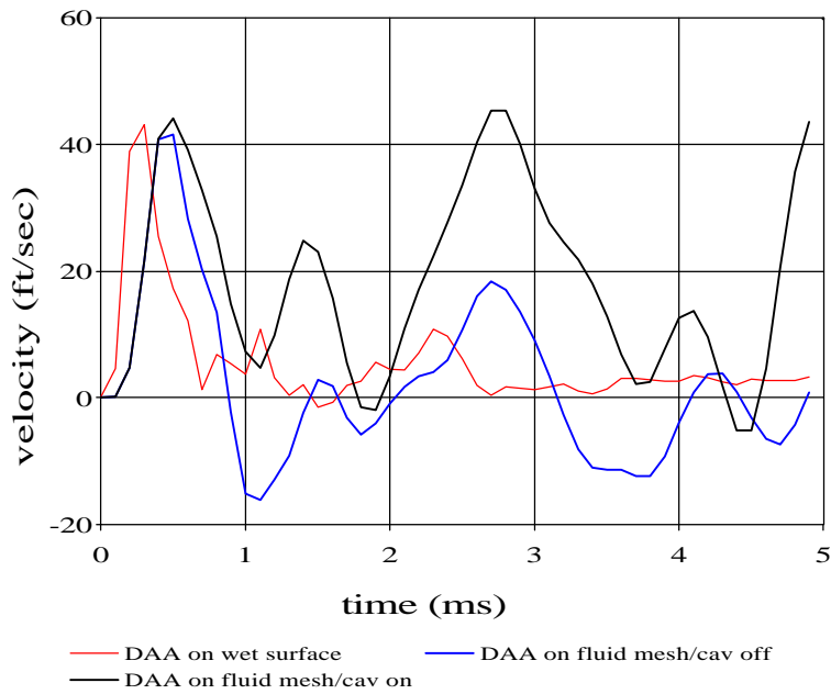
Figure 52. 3-D Model w/Offset Charge Response Comparison
